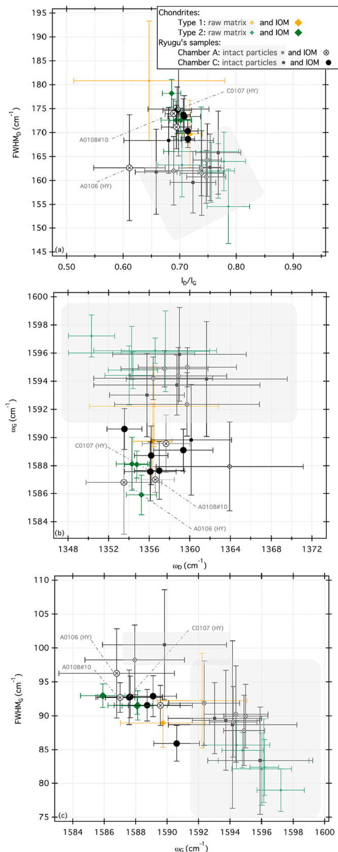
Fig. 5. Spectral parameters of Raman bands ((a) FWHM D vs. I D /I G , (b) ω G vs. ω D , (c) FWHM G vs. ω G ) obtained on IOM chemically extracted from Hayabusa2 particles (in black) and reference chondrites (type 1 CI Orgueil in yellow and type 2 CM chondrites (R1) in green). For comparison, corresponding data for intact particles and matrix fragments are reported and shaded in grey. Most of the IOM were chemically extracted at IPAG, except two of them that were extracted by H. Yabuta (HY on the graph). Averages (symbols) and standard deviations (bars) are plotted for each sample. (For interpretation of the references to colour in this figure legend, the reader is referred to the web version of this article.)
