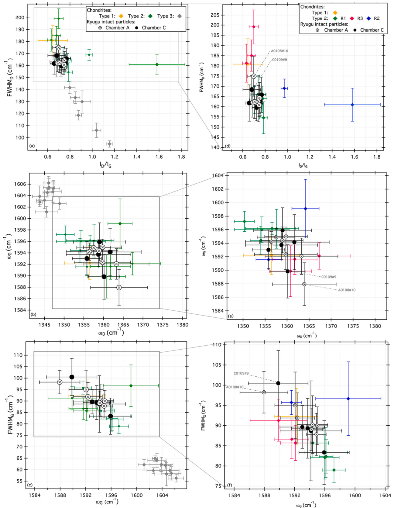
Fig. 4. Spectral parameters of Raman bands of carbonaceous materials ((a, d) FWHM D vs. I D /I G , (b, d) ω G vs. ω D , (c, f) FWHM G vs. ω G ) in the Ryugu intact particles (in black) as compared to reference chondrites (CI Orgueil in yellow, type 2 CM chondrites in green on Figs. a, b, c and in green, magenta and blue on Figs. d, e, f and type 3 chondrites in grey). The three colors for type 2 chondrites (“R1” in green, “R3” in magenta, and “R2” in blue) reflect variable extents of short-duration heating (see Section 4.2. for explanation and Quirico et al., 2018). Averages (symbols) and standard deviations (bars) are plotted for each sample. (For interpretation of the references to colour in this figure legend, the reader is referred to the web version of this article.)
